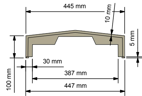
Joint Elevation
