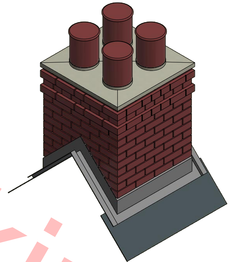
Auxiliary View ( 1 : 20 )
