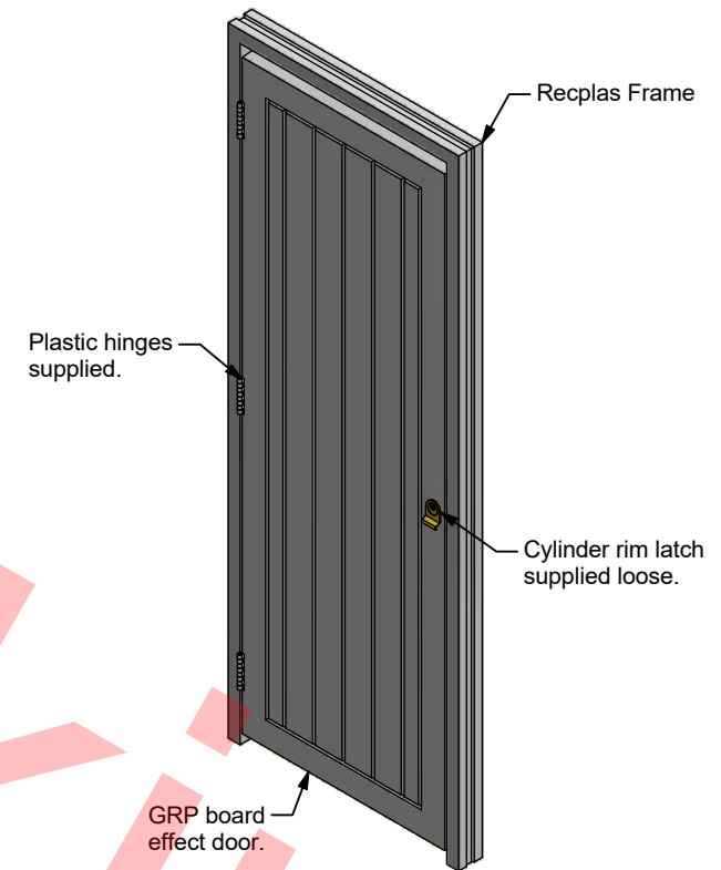
Auxiliary View ( 1 : 20 )
