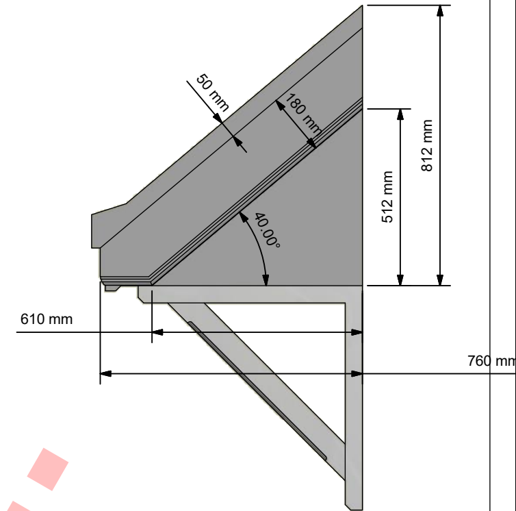
Side View ( 1 : 15 )
