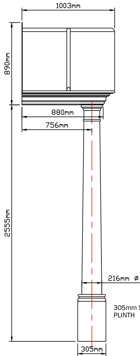
SIDE ELEVATION
