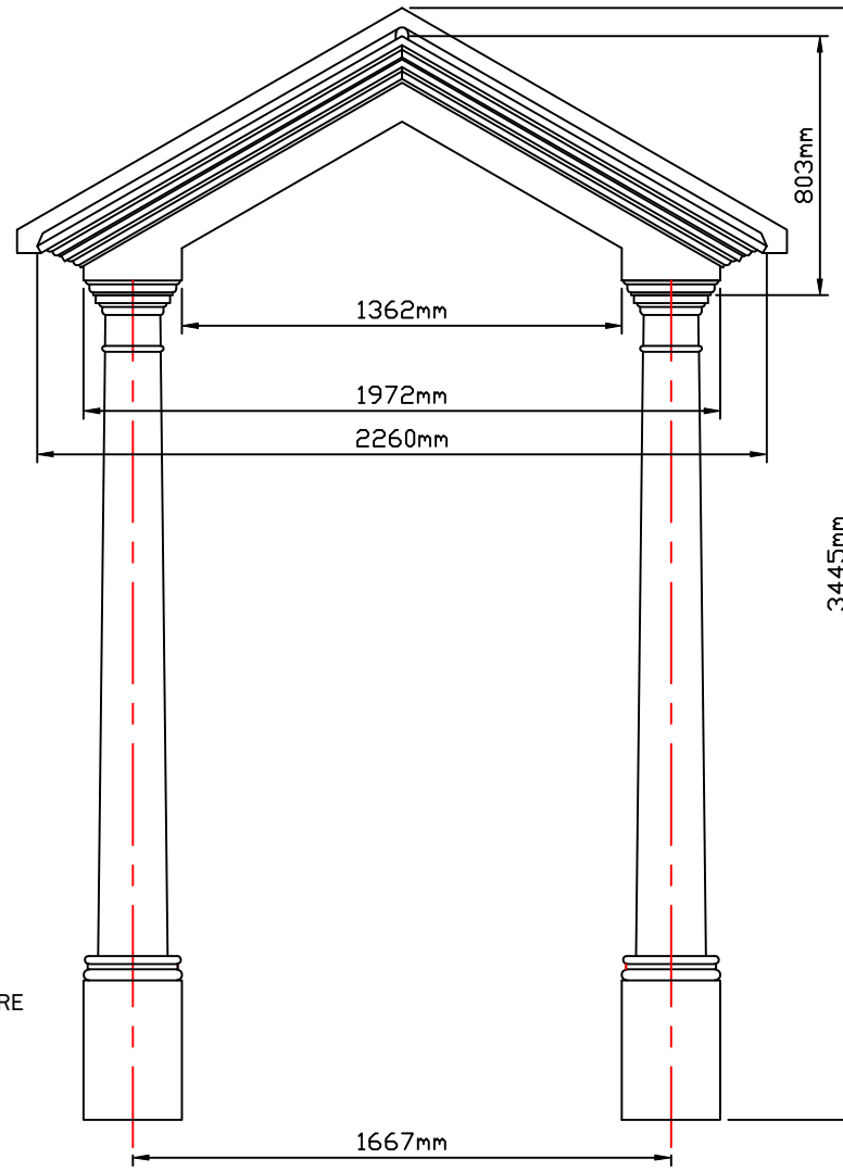
FRONT ELEVATION
