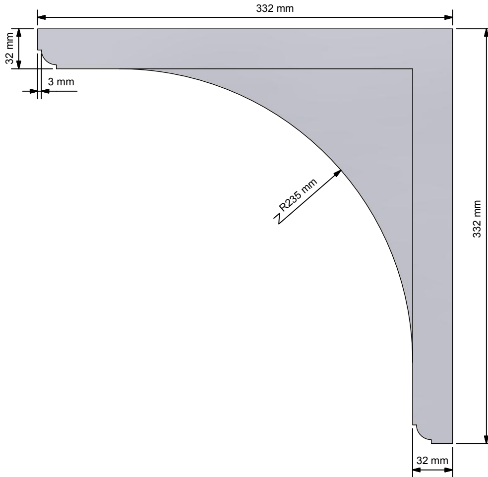
Side Elevation ( 1 : 3 )
