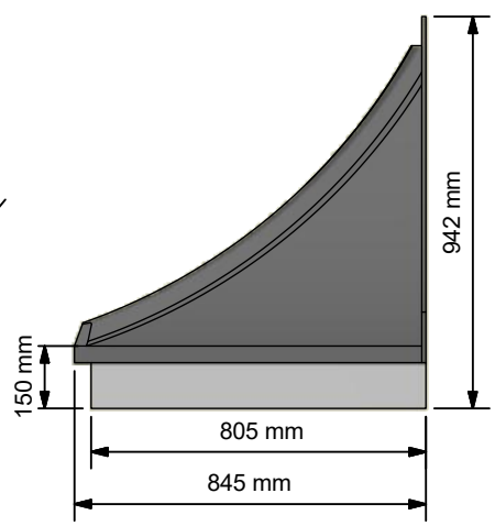
Side Elevation ( 1:20 )
