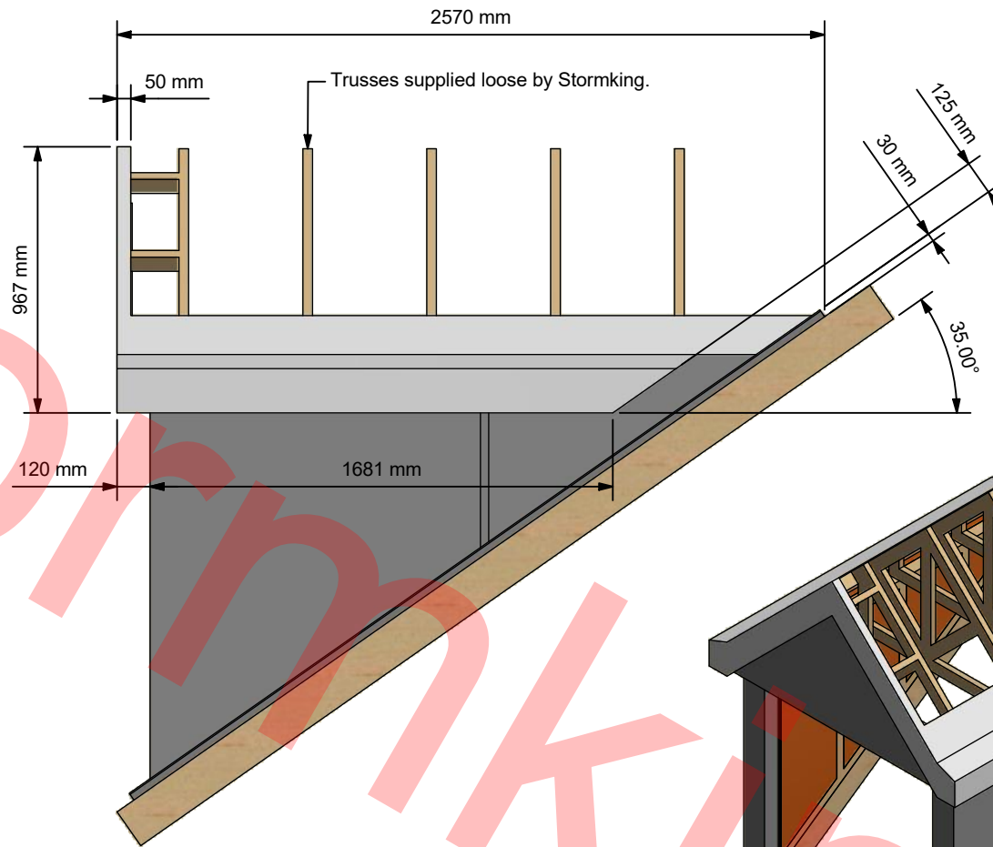
Side Elevation ( 1:25 )
