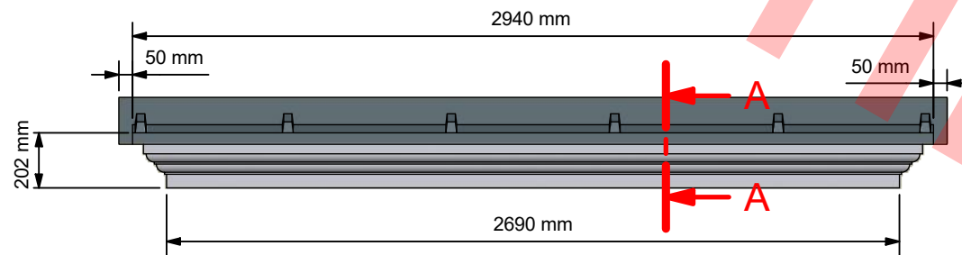
Front Elevation ( 1:25 )
