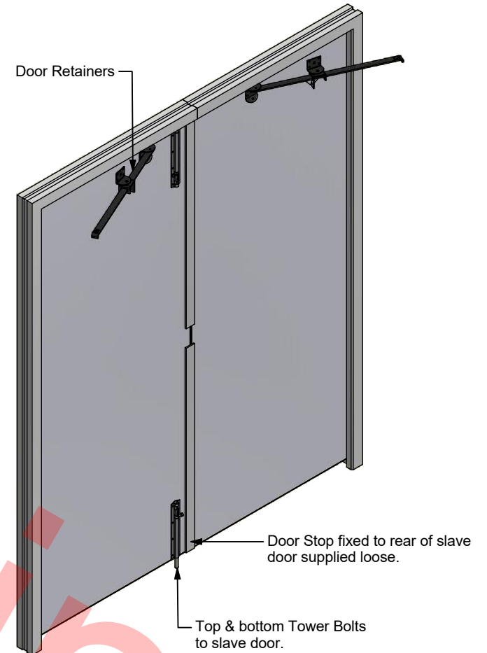
Auxiliary View On Rear Of Doors ( 1 : 20 )
