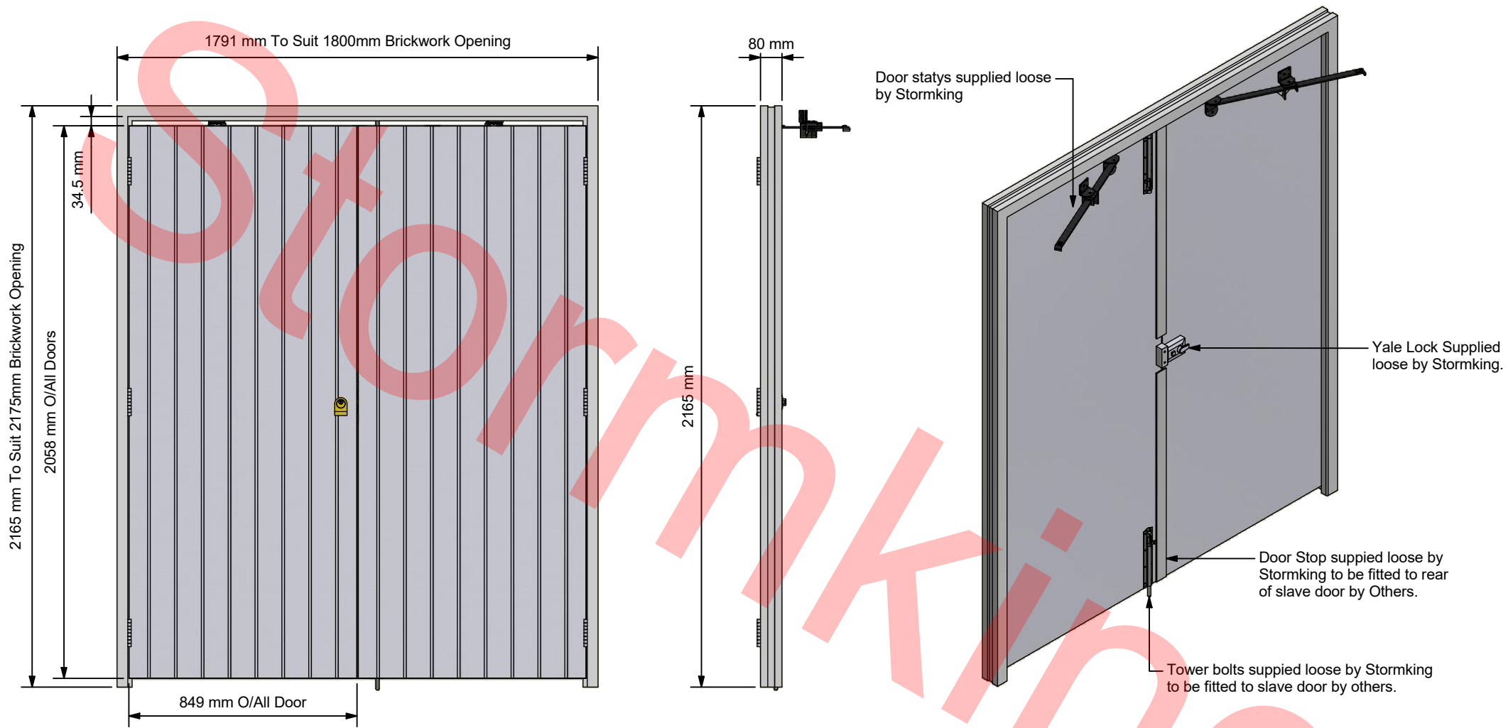
Front Elevation ( 1:20 )
