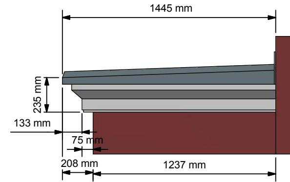
Side View ( 1 : 25 )
