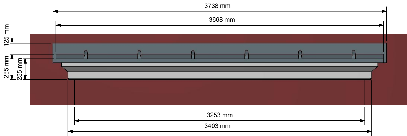
Front Elevation ( 1 : 25 )
