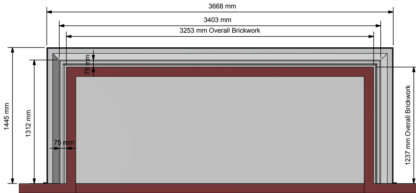
Reflected Plan View ( 1 : 25 )
