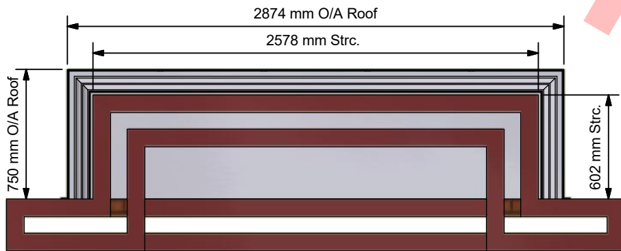
Reflected Plan Elevation ( 1 : 30 )
