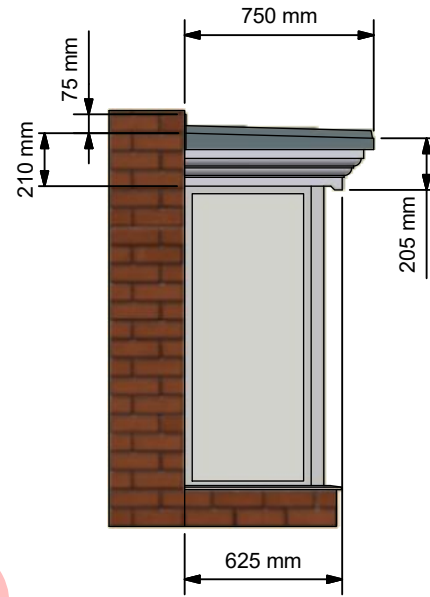
Side Elevation ( 1 : 30 )
