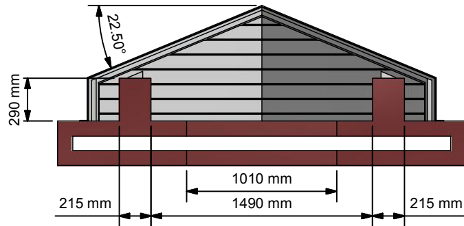
Reflected Plan Elevation ( 1 : 35 )
