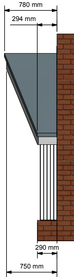
Side Elevation ( 1 : 35 )
