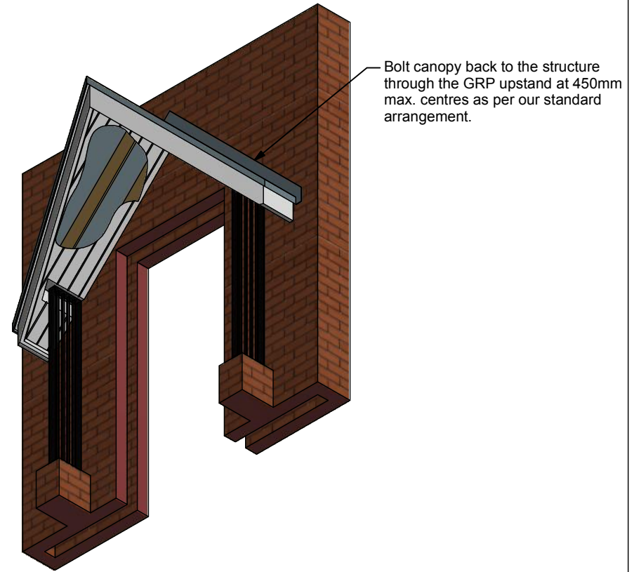
Auxiliary View ( 1 : 35 )
