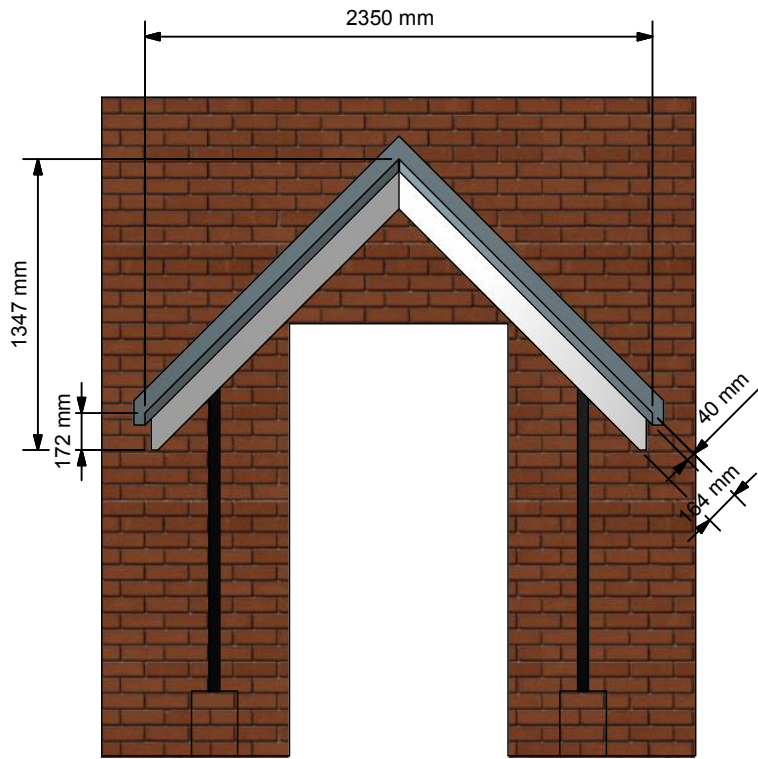
Front Elevation ( 1 : 35 )
