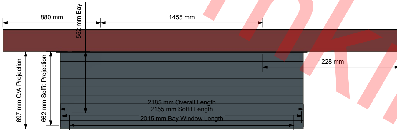
Reflected Base View ( 1 : 20 )
