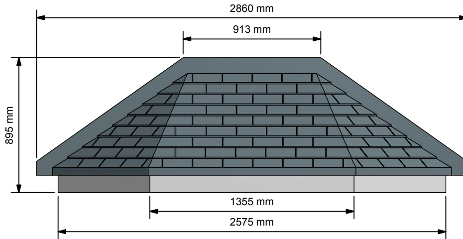
Front Elevation ( 1:25 )
