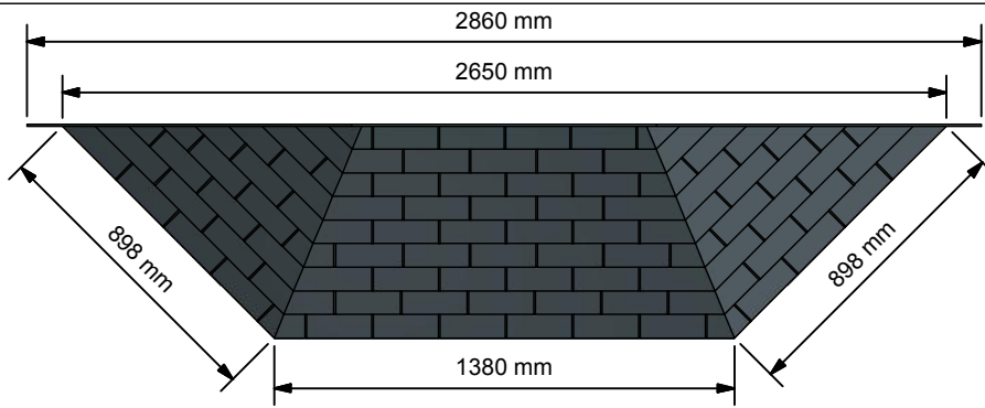
Plan View ( 1:25 )
