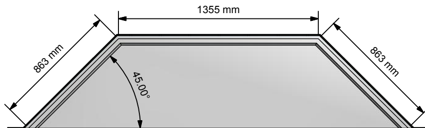
Reflected Plan View ( 1:25 )
