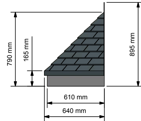
Side Elevation ( 1:25 )
