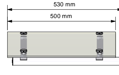
Side Elevation
