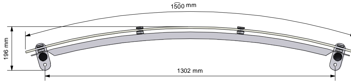
Front Elevation ( 1 : 10 )
