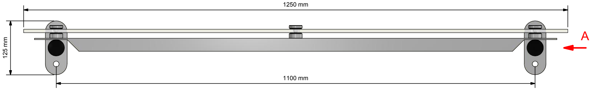
Front Elevation ( 1 : 5 )
