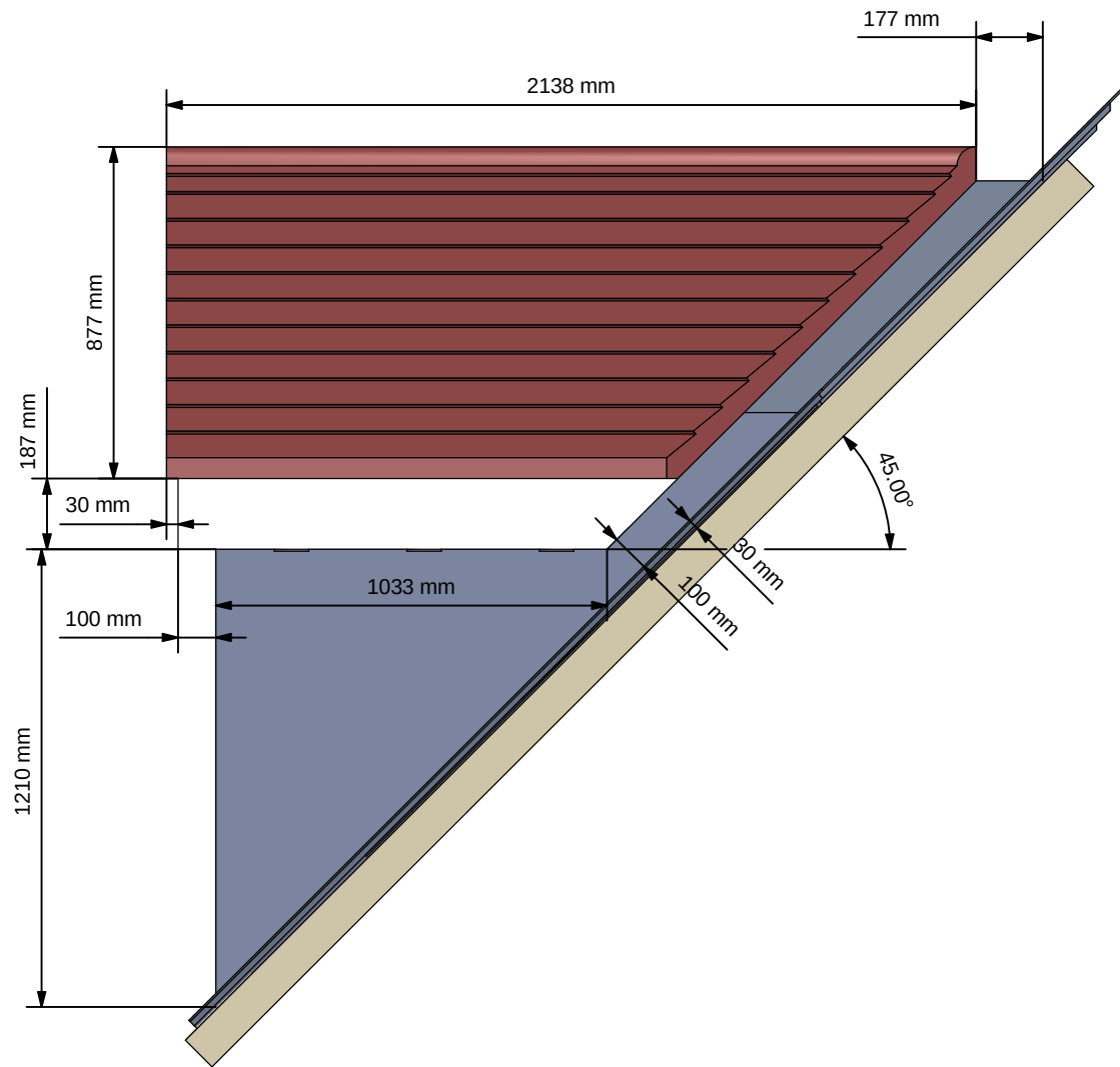
Side Elevation
