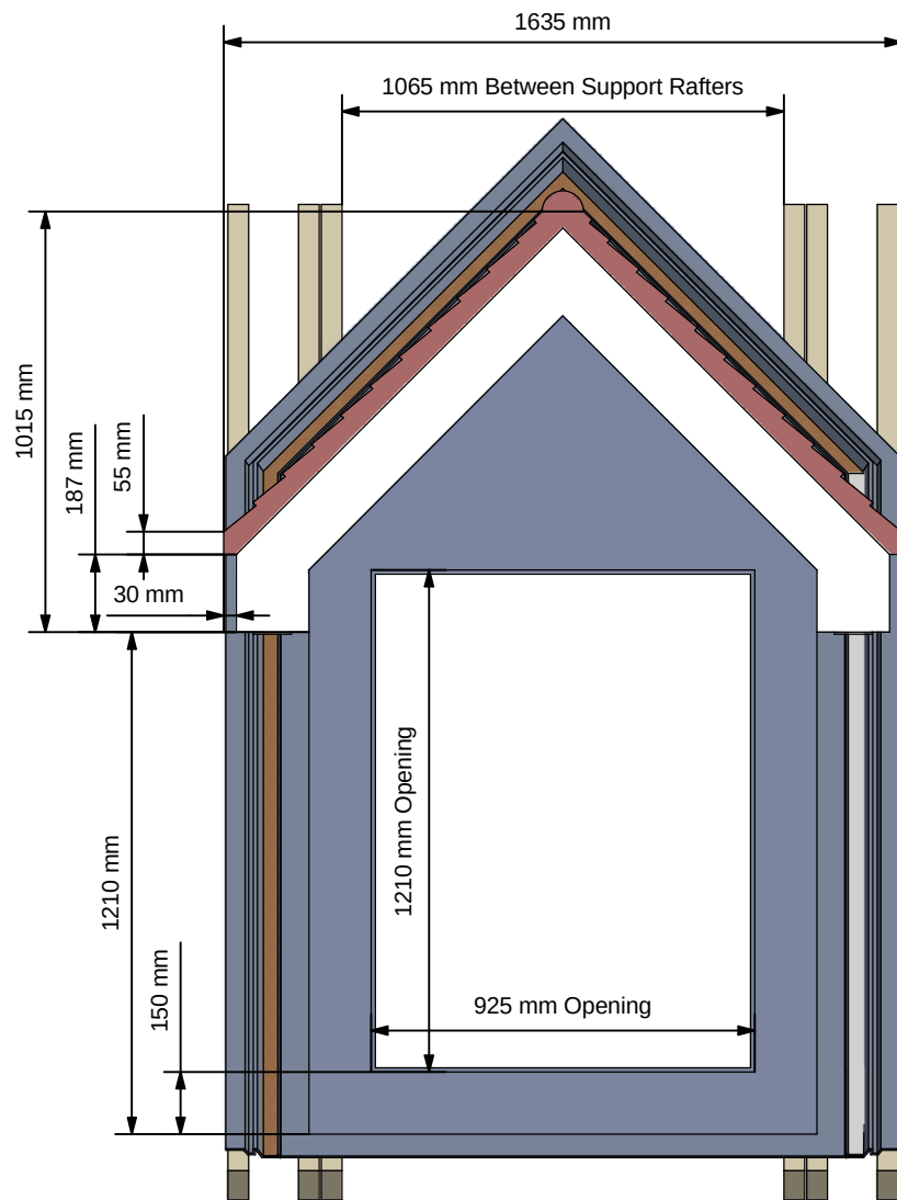
Front Elevation ( 1 : 20 )
