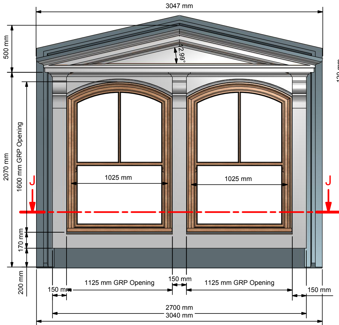
Front Elevation ( 1 : 25 )
