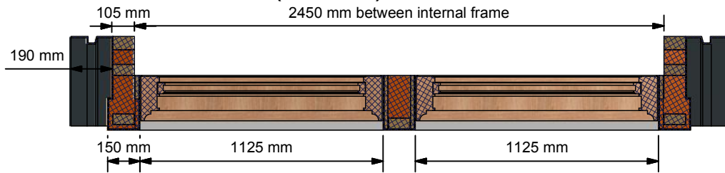
Front Elevation ( 1 : 25 )
